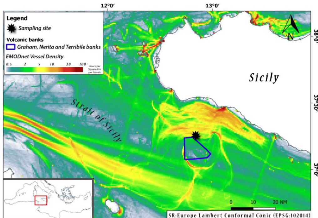
Figure 1: Map of the DWRS sampling site with overlapped shipping density.
